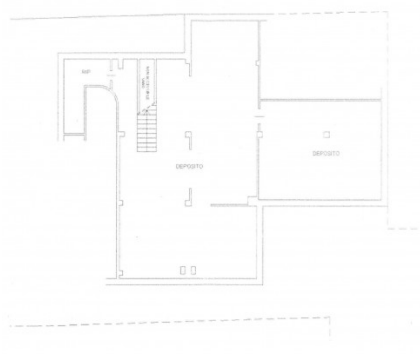
PIANO INTERRATO H ml. 2.80
